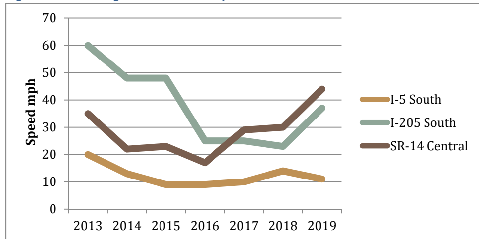
Figure 50: Morning Bi-State Travel Speeds
