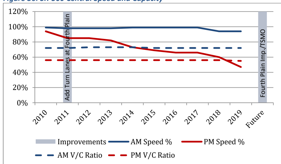
Figure 36: SR-500 Central Speed and Capacity
