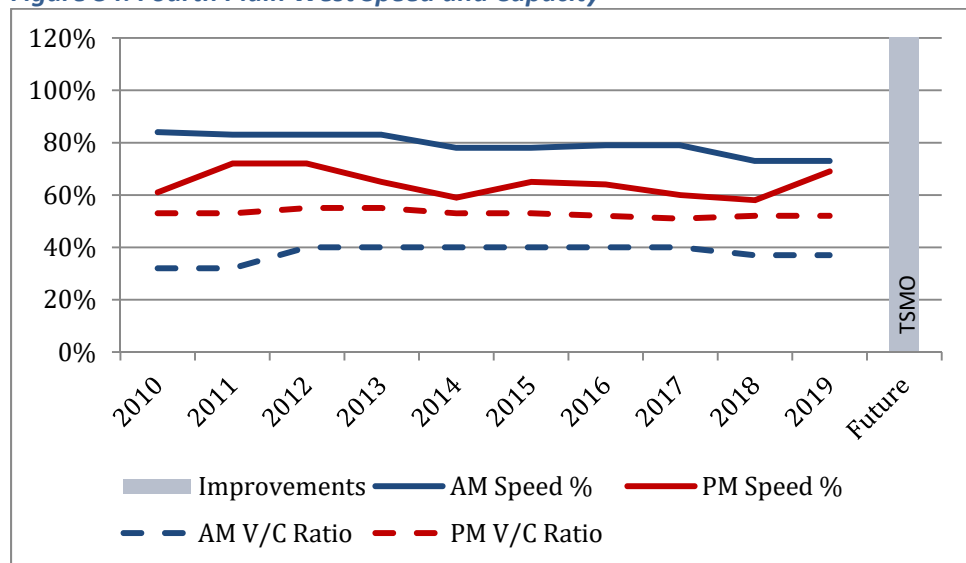
Figure 34: Fourth Plain West Speed and Capacity
